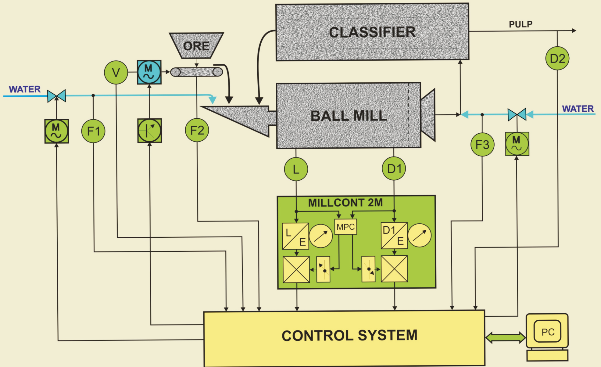
ORE GRINDING PROCESS CONTROL SYSTEM
