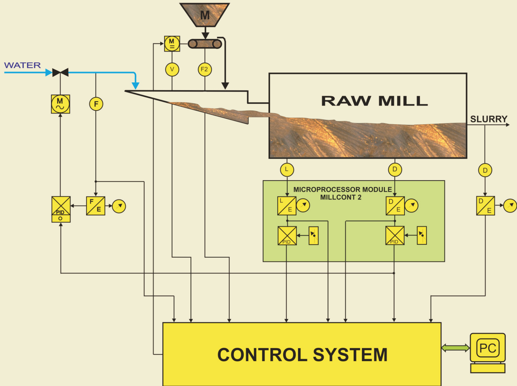
MICROPROCESSOR CONTROL SYSTEM OF WET GRINDING RAW MILL
