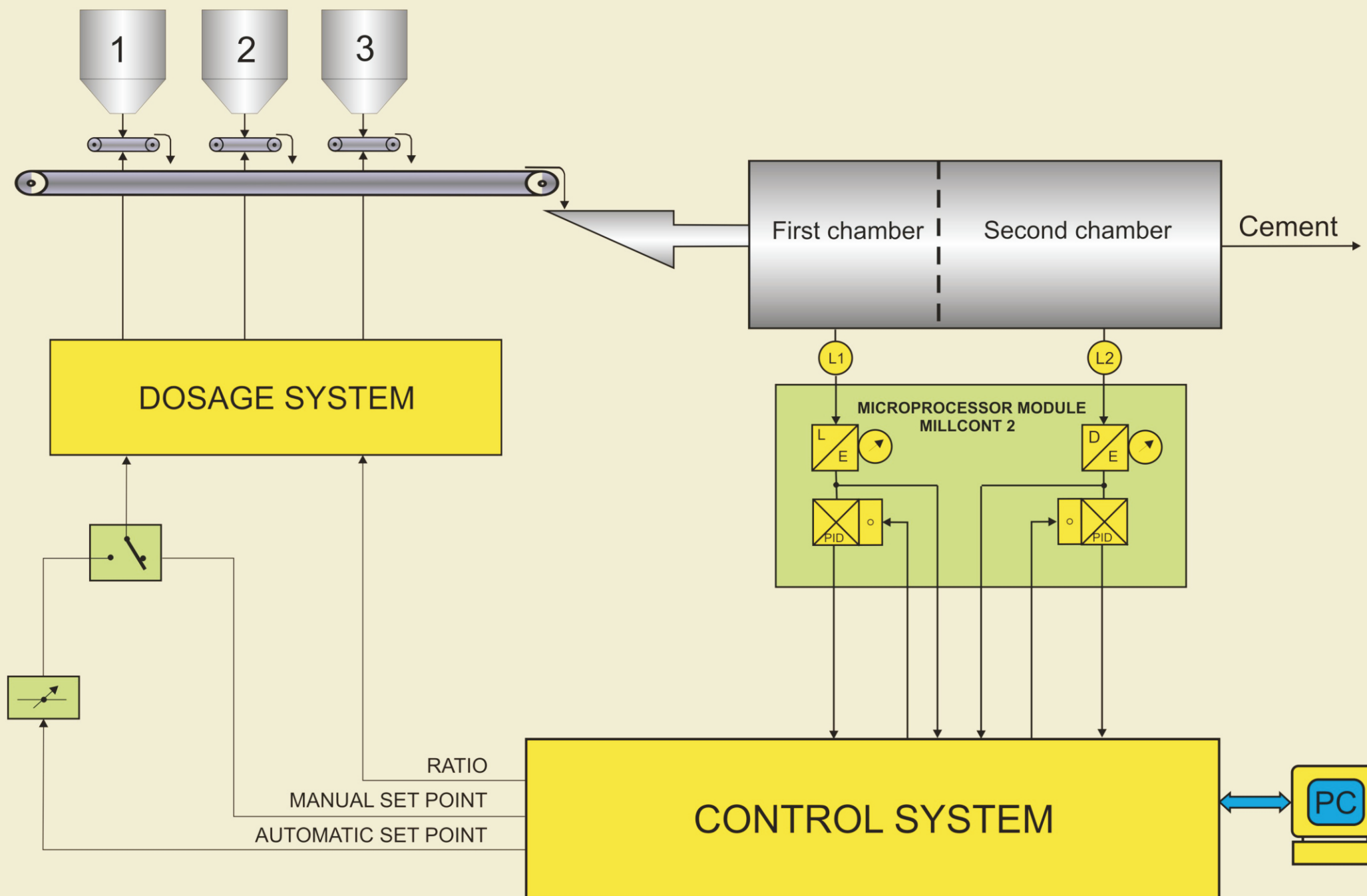
GRINDING PROCESS CONTROL SYSTEM OF OPEN CYCLE MILL (IRAN, Hormozgan cement plant)
