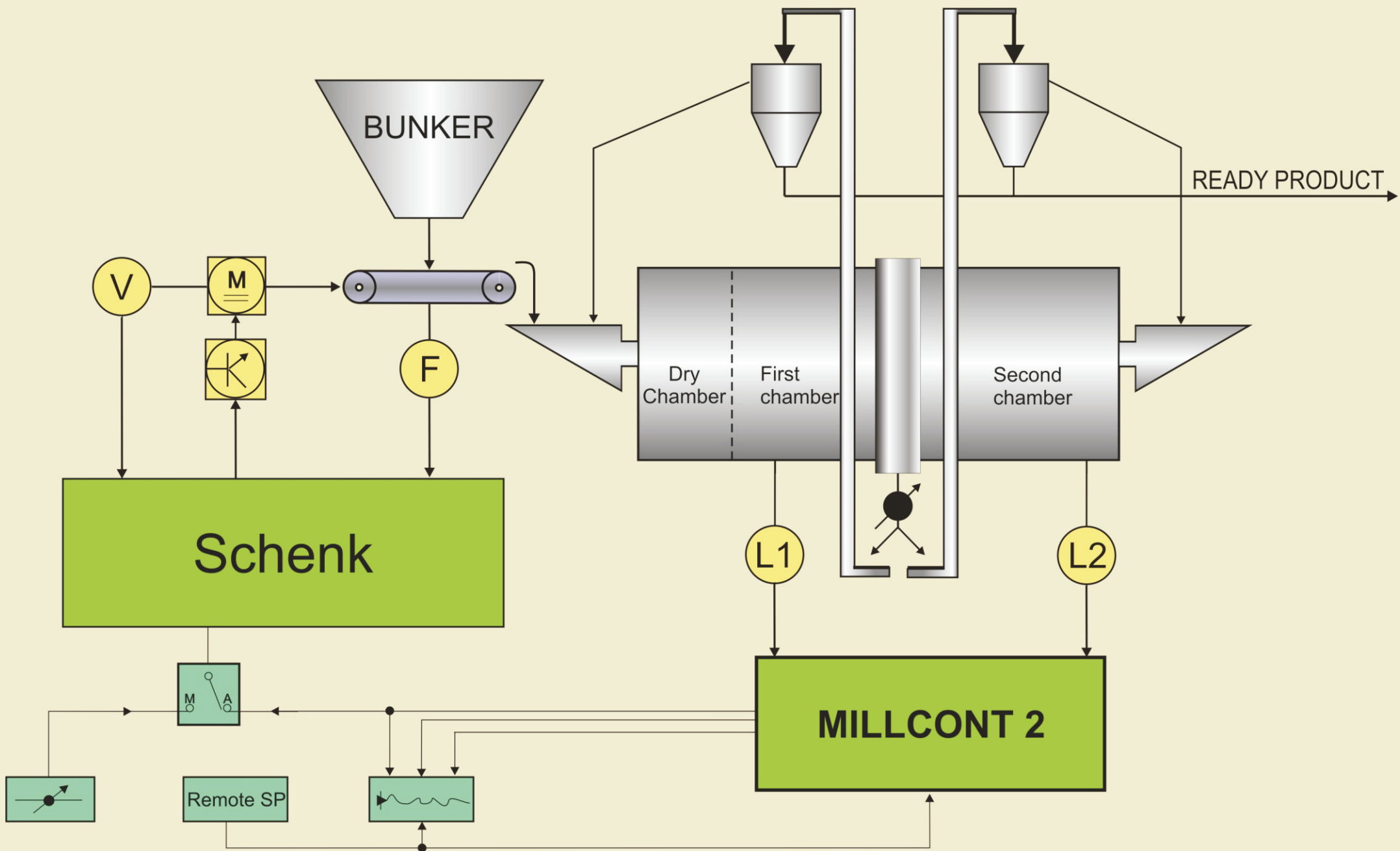
GRINDING PROCESS CONTROL SYSTEM OF TWO-STAGE RAW MILL (IRAN, Abyek cement plant)
