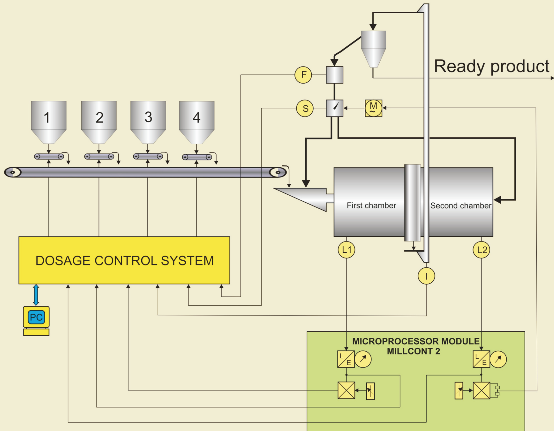
GRINDING PROCESS CONTROL SYSTEM OF TWO-STAGE RAW MILL
