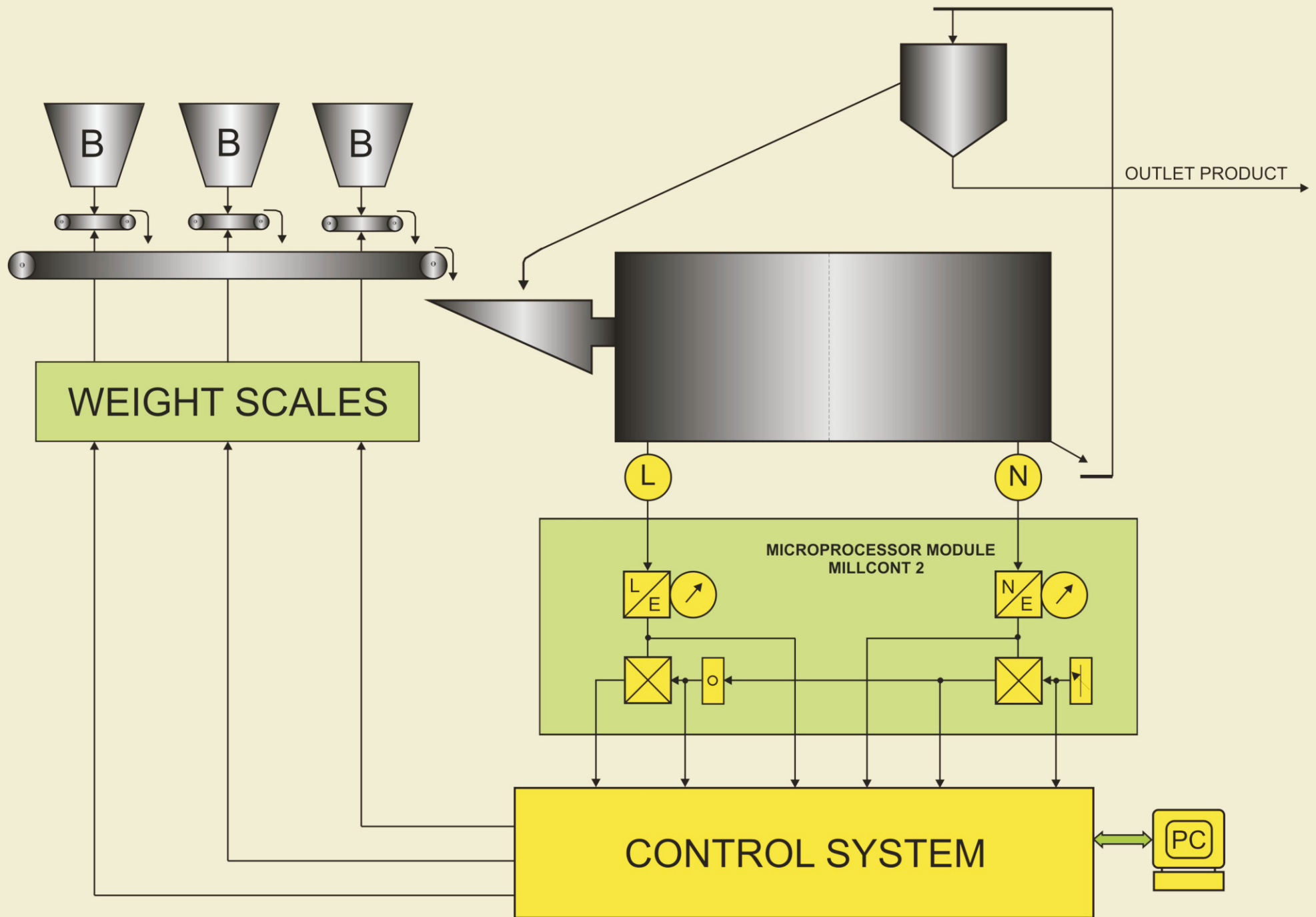
GRINDING PROCESS CONTROL SYSTEM OF SINGLE-STAGE SEPARATOR MILL
